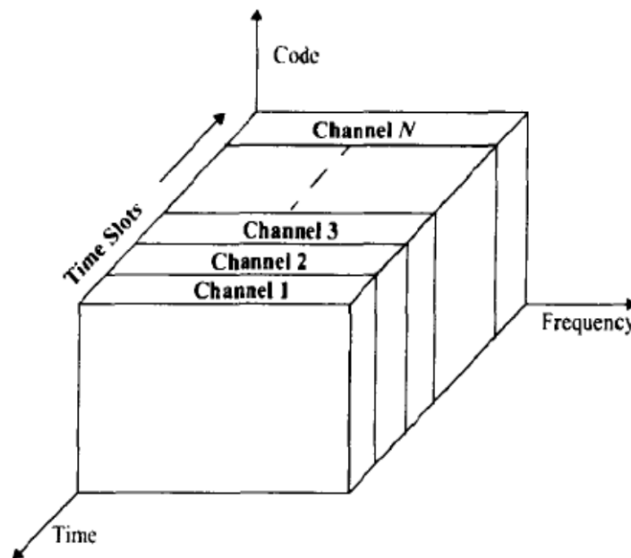
Figure 8.3 TDMA scheme where each channel occupies a cyclically repeating time slot.
