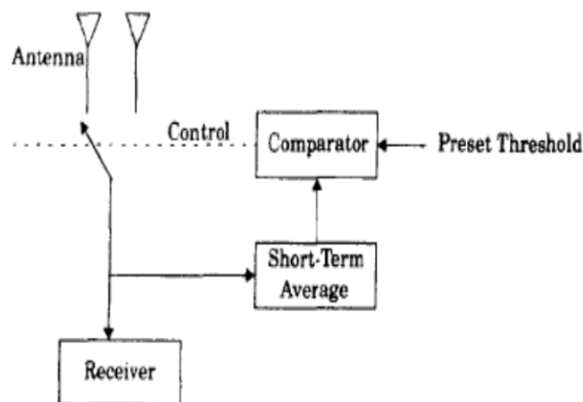
Fig.8 block diagram of scanning diversity
