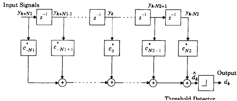
Fig.1 Structure of linear transversal equalizer
