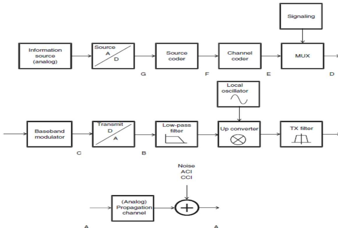
Fig:Block diagram of a digital transmitter chain for mobile communications
