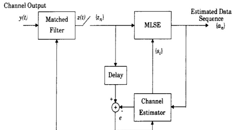
Fig.5 Structure of MLSE with adaptive matched filter
