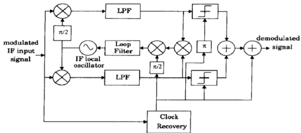
Fig.3.7 Block diagram of GMSK receiver
