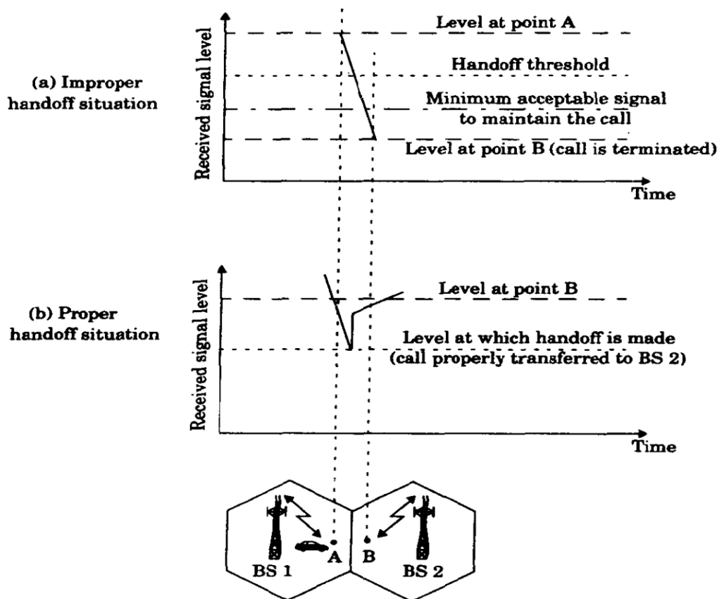
Fig 2.2 Illustration of handoff strategies
