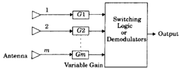
Fig 7. Block diagram of selection diversity
