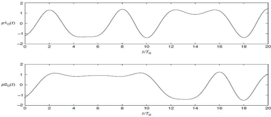
Fig: QAM Pulse Sequence
