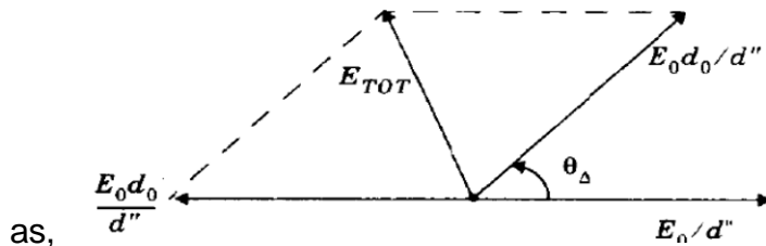
Fig3. Phasor diagram of LOS, ground reflected and total received E-field
