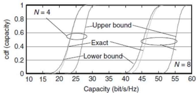
Fig: Exact capacity, upper bound, and lower bound of a multiple-input-multiple-output system
