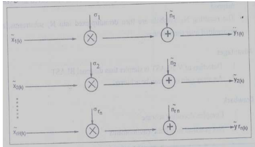
Fig:SVD Precoding x—channel input y—channel output
