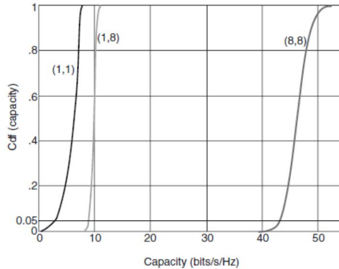
Fig: Cumulative distribution function of capacity for 1 \times 1 , 1 \times 8 , and the 8 \times 8 optimum scheme.
