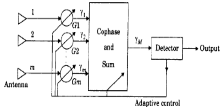
Fig.9 Maximal ratio combiner
