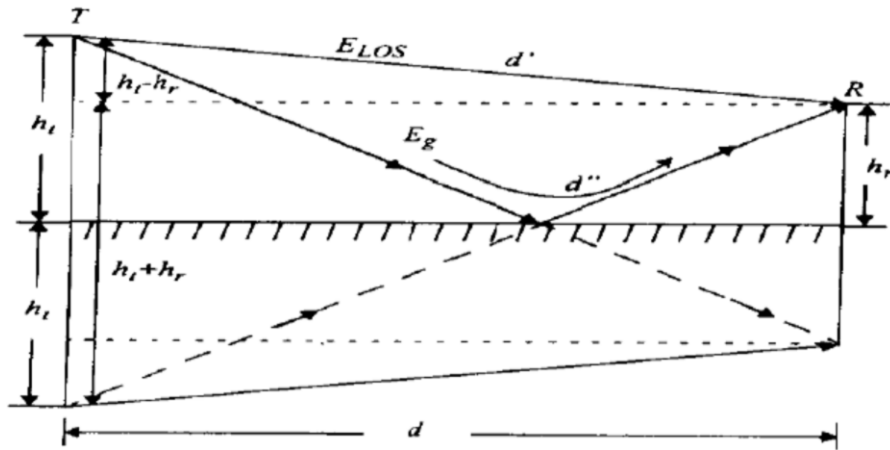
Fig2. Geometry for find the path difference between LOS and ground reflected paths.
