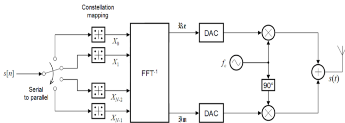
Fig: OFDM Transmitter block diagram
