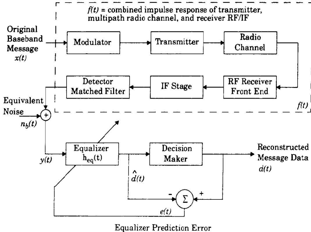
Fig: Adaptive Equalization Block diagram
