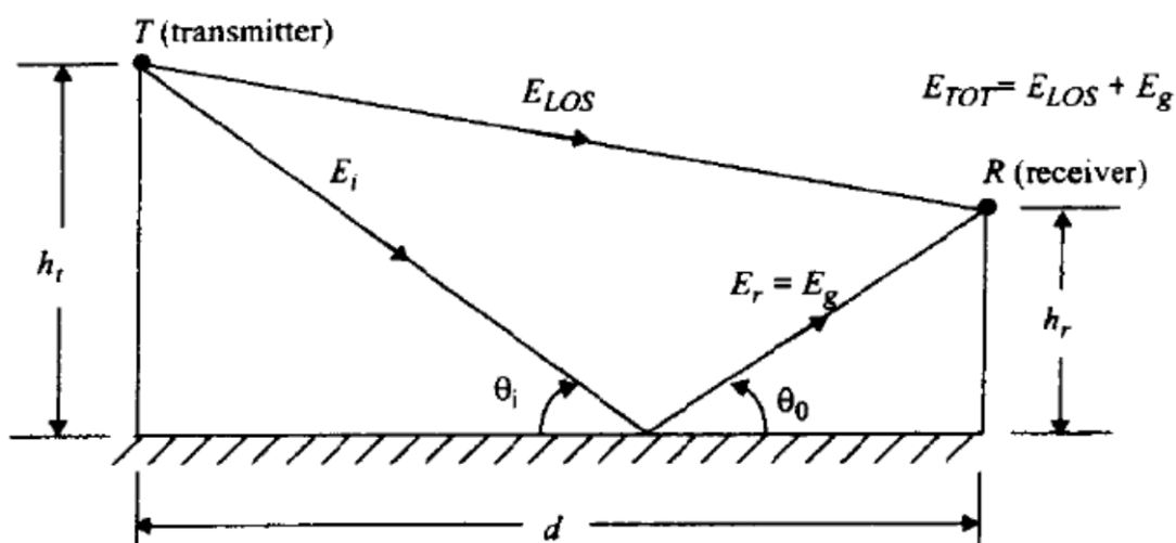
Fig1. Two-ray ground reflection model
