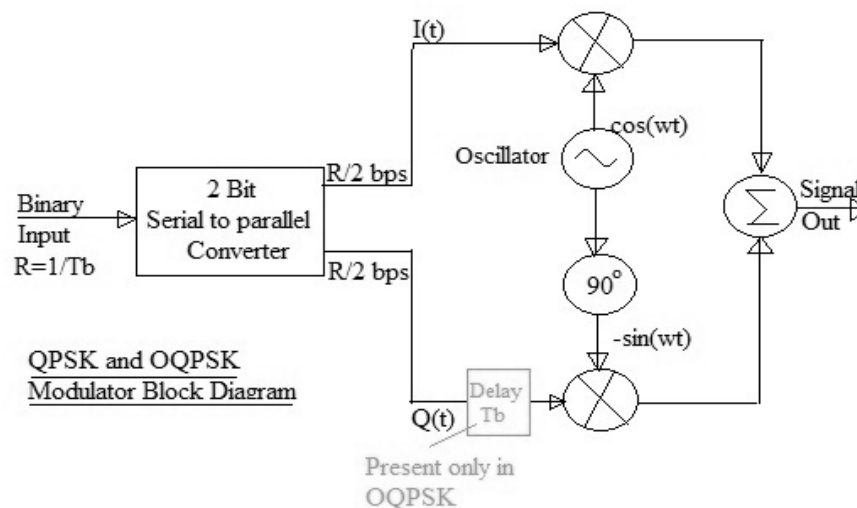
Fig: Difference b/w QPSK and OQPSK
