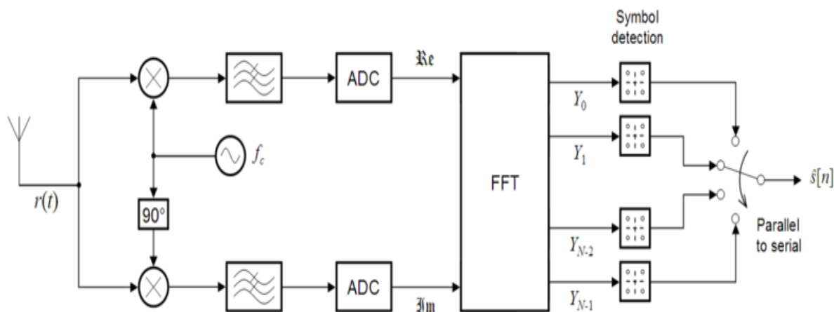
Fig: OFDM Receiver block diagram
