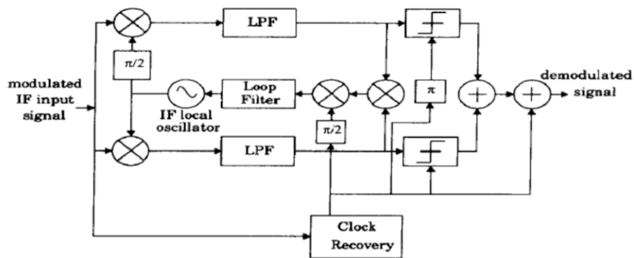
Fig.3.7 Block diagram of GMSK receiver
