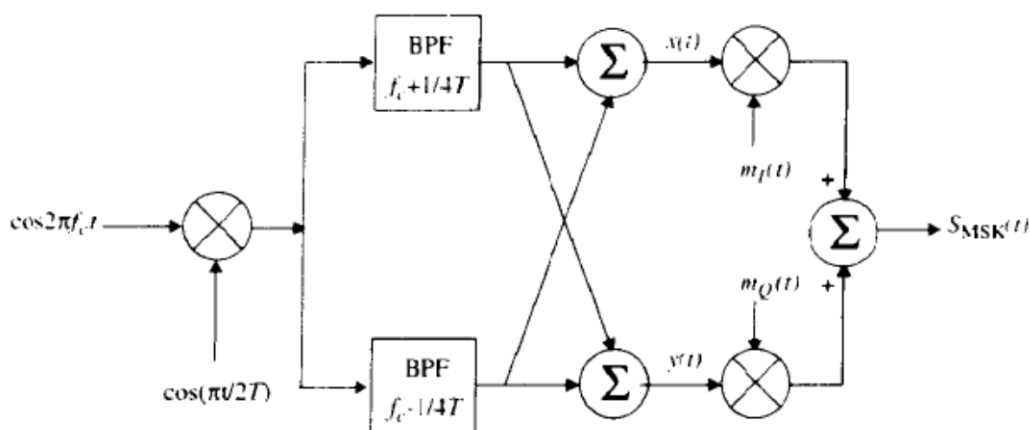
Fig.3.3 Block diagram of MSK Transmitter
