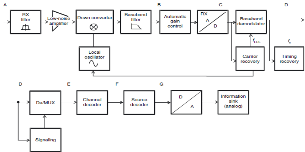
Fig:Block diagram of a digital receiver chain for mobile communications
