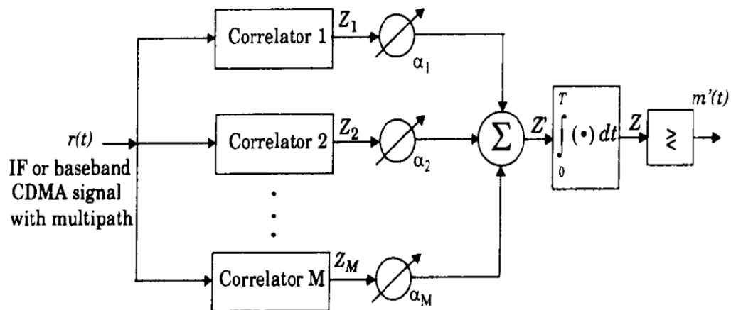
Fig:Rake Receiver
