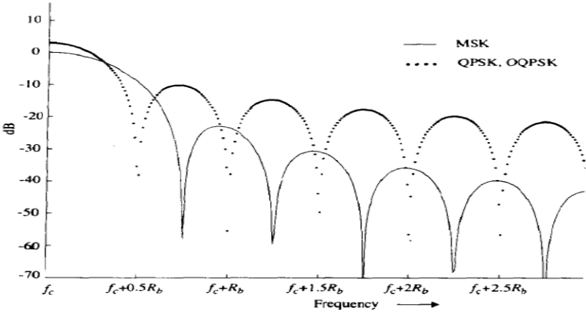
Fig.3.2 power spectrum of MSK
