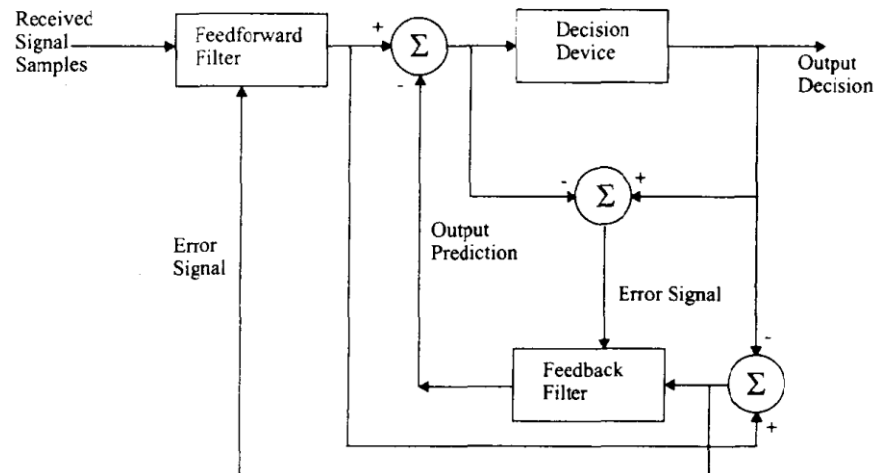
Fig.4 Predictive decision feedback equalizer
