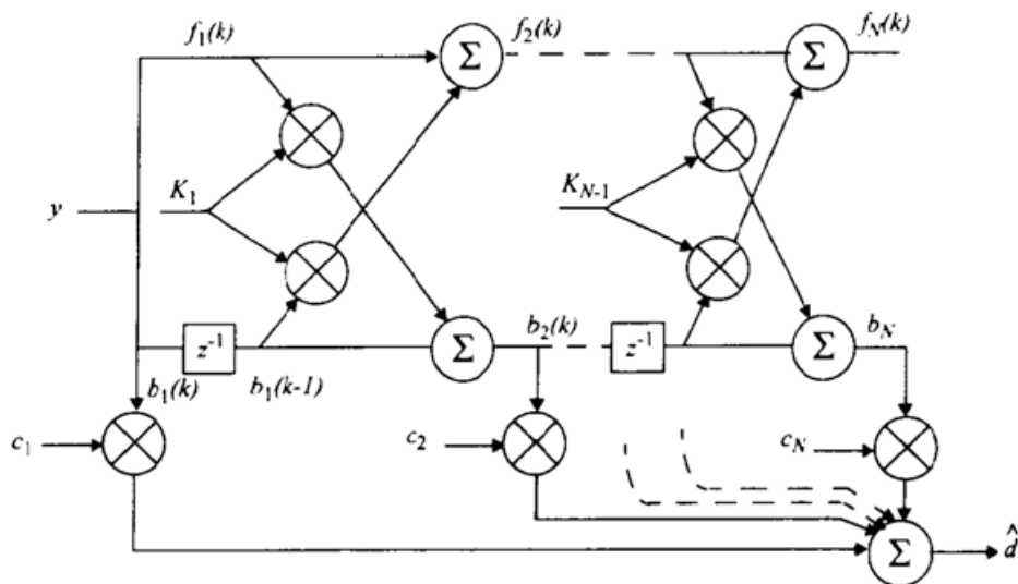
Fig.2 Structure of Lattice filter
