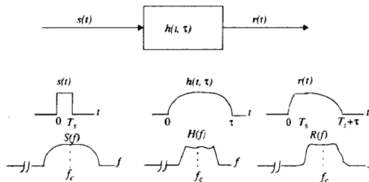
Figure 4.13 Frequency selective fading channel characteristics.
