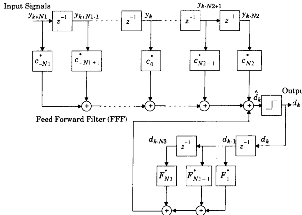
Fig.3 Direct form of Decision feedback equalizer
