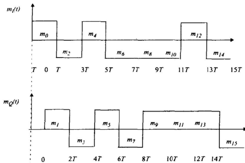
Fig.3.1 Offset waveforms
