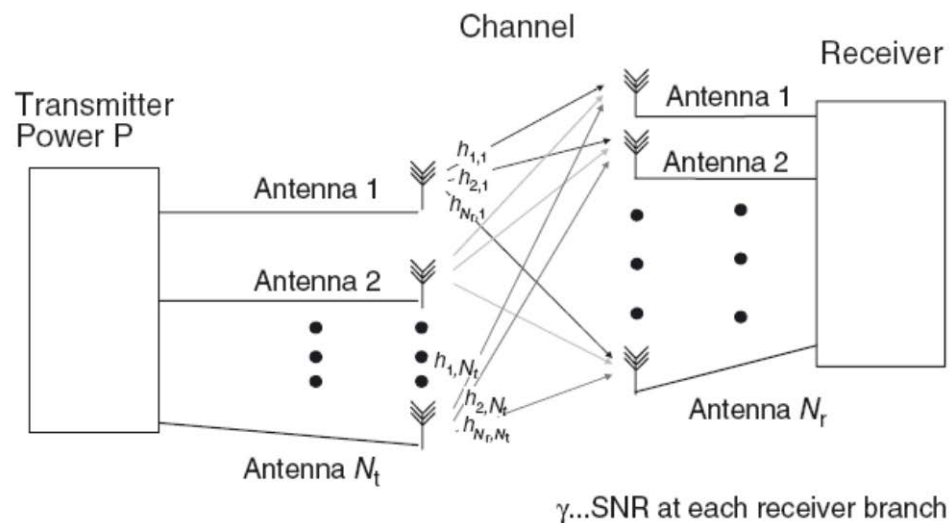
Figure 20.10 Block diagram of a multiple-input multiple-output system.
