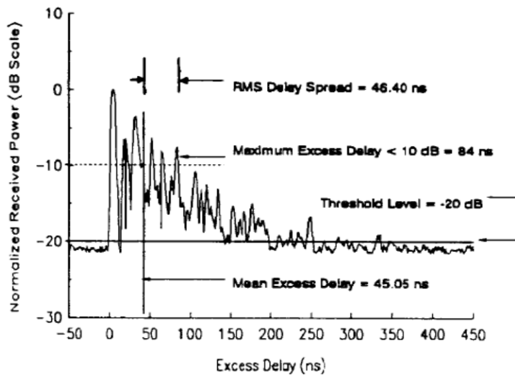
Figure 4.10 Example of an indoor power delay profile; rms delay spread, mean excess delay, maximum excess delay (10 dB), and threshold level are shown.
